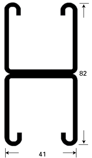
CH103 Weight 5.2 Kg/m
