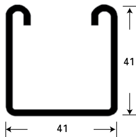
CH101 Weight 2.6 Kg/m
