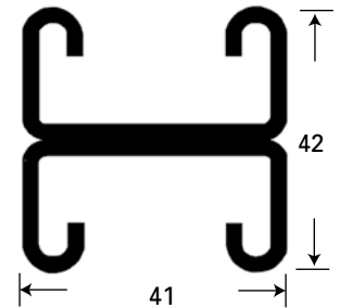
CH105 Weight 3.6 Kg/m
